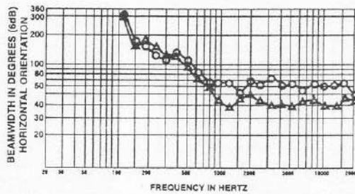
FIGURE 5 — MTH-2.5/64B Directivity vs. Frequency
